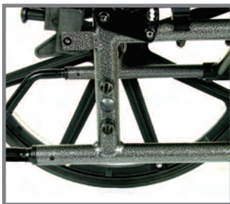
Adjustable Axle Positions Three seat height positions and the ability to add a fixed tilt allow for greater flexibility.
